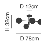
D 12cm 77-8179 KQ S0982-4 4xE27, max 60W, 230V
