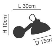
77-4500 YQ-4004 1xE27 max 40W
