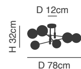
D 12cm 77-8179 KQ S0982-4 4xE27, max 60W, 230V
