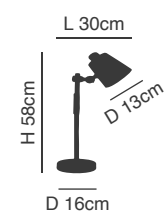
77-4496 YQ-25110 1xE27, max 40W, 230V
