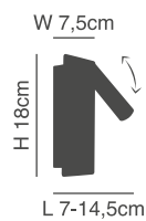
77-3567-36 SE 129-1AW LED, 3W, 230V
