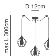
77-8748-72 SE21-BL-B10-BL3-GR1 3xE27, max 60W, 230V
