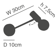
77-8274-26 SE21-BL-22 1xE27, max 60W, 230V
