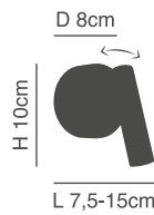
77-3517-23 SE-127-1AN LED, 1xE27, 3W, 230V
