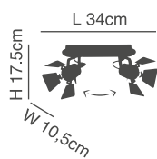
77-2209-80 GU12015A-2B 2xGU10, max 50W, 230V
