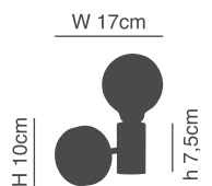
77-8253-22 SE21-BL-16 1xE27, max 60W, 230V
