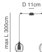
77-8756-51 SE21-BL-B10-BL2-GR2 2xE27, max 60W, 230V
