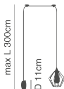
77-8894-30 SE21-BL-B10-BL1W-GR1 1xE27, max 60W, 230V
