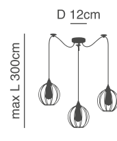
77-8755-72 SE21-BL-B10-BL3-GR2 3xE27, max 60W, 230V
