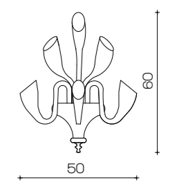
Art 1965/A6 ø 50 cm H 60 cm 6 x G9 x 40W
