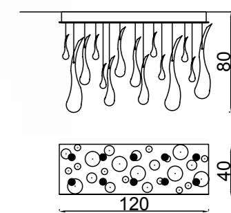
Art.2062/Steel L 120 x 40 cm H 80 cm 10 x GU10 x 40W (Available IP65)
