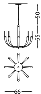
Art.2071/CH8/BI ø 66 cm H 55 cm +50 cm steel cable 8 xG9 x Led 10W
