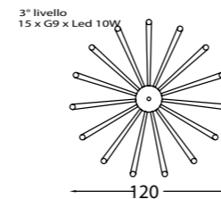
Art. 2071/CH30/BI ø120 cm H 120 cm +50 cm steel cable 30 xG9 x Led 10W
