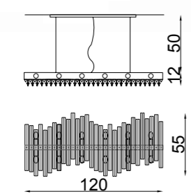
Art.2055/NN L 120 x 55 cm H 12 cm +50 cm Steel cable 12 x E14 x 40W
