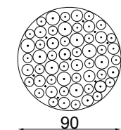
Art. 2078/Steel ø 90 cm H 48 cm 18 x G9 x 25W Steel
