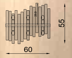
Art. 2054/A/NN L 60 cm H 55 cm Sp12 cm 6 x E14 x Led 5 W
