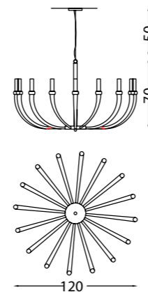
Art. 2071/CH16/BI ø 120 cm H 70 cm +50 cm steel cable 16 xG9 x Led 10W
