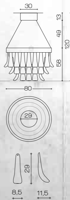
Art 1939 Chandelier ø 80 cm H 58 cm + Ceiling plate H 13 cm ø 30 cm with 3 GU 10 Led 10W H at 120 cm + Strip Led Colour light 2700 K° Lumen 8550
