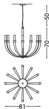
Art. 2071/CH12/BI ø 81 cm H 70 cm +50 cm steel cable 12 xG9 x Led 10W
