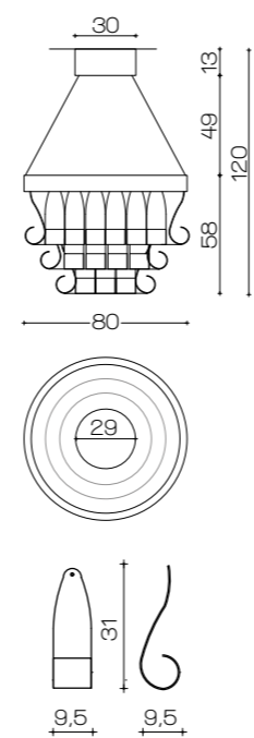
Art 1937 Chandelier ø 80 cm H 58 cm + Ceiling plate H 13 cm ø 30 cm with 3 GU 10 Led 10W H at 120 cm + Strip Led Colour light 2700 K° Lumen 8550
