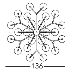
Art. 2129/CH36/SG Ø 136 cm - H 107 cm 36 x G9 x Led 10W
