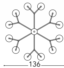
Art. 2129/CH12/SG Ø 136 cm - H Tot. 100 cm 12 x G9 x Led 10W
