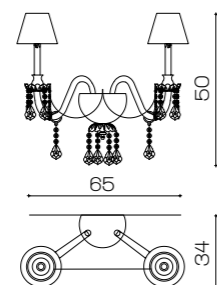
Art. 1761/A2 ø 65 cm H 50 cm Pø 35 cm 2 x E14 x Led
