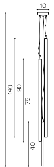
Art. 2138/CH3 ø 10 cm Kg 8 H 140 cm 3 x G9 x Led
