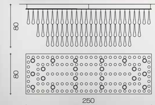
Art. 2016/STEEL L 250 x 80 cm H 80 cm 22 x GU10 x Led 5W (Available IP65)
