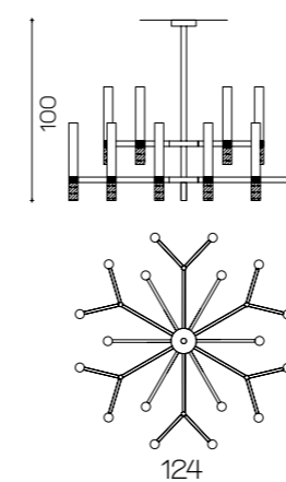
Art. 2173/CH18+18 ø 124 cm H 100 cm 36 x G9 x Led
