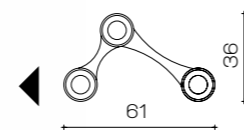
Art. 2197/BI/GOLD L 61 x 36 cm H 3 cm H tot 25 cm G x 53 3 x 11W Led ø int. 75 mm
