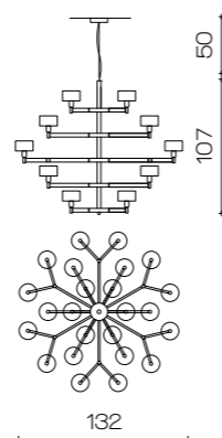
Art. 2127/CH36 ø 132 cm H 107 cm Pø 14 cm 36 x E14 x Led
