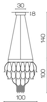
Art. 1984/P ø 100 cm H 100 cm +Ceiling plate ø 30 cm H 8 cm Steel cable 140 cm 9 x E27 x 60W +3 GU10 Led 10W
