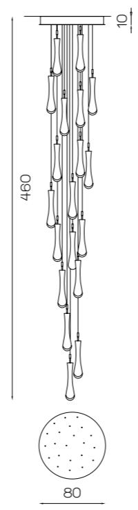
Art. 2182 ø 80 cm H 460 cm 22 x G9 x Led
