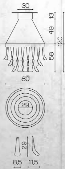
Art. 1939 Chandelier ø 80 cm H 58 cm +Ceiling plate H 13 cm ø 30 cm with 3 GU10 Led 10W H tot. 120 cm +Strip Led Colour light 2700 K° Lumen 8550
