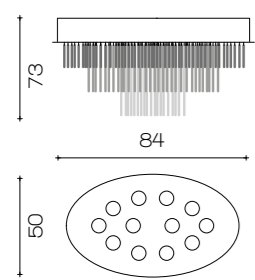
Art. 2027/OVALE/STEEL L 84 x 50 cm H 40 cm 12 x GU10 x Led 10W
