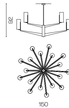
Art. 2169/CH9 ø 150 cm H 92 cm Pø 12 cm 18x E14 x Led
