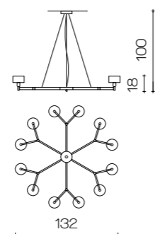
Art. 2127/CH12 ø 132 cm H 18 cm H tot. 100 cm Pø 14 cm 12 x E14 x Led
