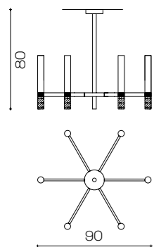
Art. 2173/CH6+6 ø 90 cm H 80 cm 12 x G9 x Led
