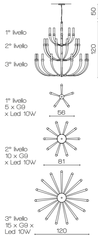
Art. 2071/CH30/BI ø 120 cm H 70 cm +50 cm steel cable 30 x G9 x Led 10W
