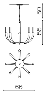
Art. 2071/CH8/BI ø 66 cm H 55 cm +50 cm steel cable 8 x G9 x Led 10W
