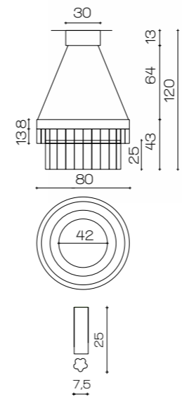
Art. 1960 ø 80 cm H 43 cm +Ceiling plate H 13 cm ø 30 cm with 3 GU10 Led 10W H tot. 120 cm Colour light 2700 K° Lumen 8550
