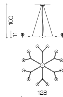
Art. 2130/CH12 ø 128 cm H 11 cm H tot. 100 cm 12 x G9 x Led 10W
