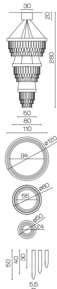
Art. 1961/LU ø 120 cm H 260 cm +Ceiling plate H 20 cm ø 30 cm with 3 GU10 Led 10W +Strip Led Colour light 2700°K Lumen 16530
