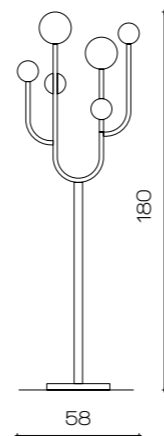
Art. 2164/FL L 58 x 65 cm H 180 cm 6 x G9 x Led
