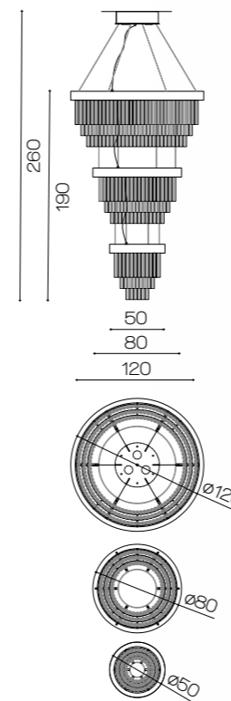
Art. 1972 ø 120 cm H 190 cm +Ceiling plate H 20 cm ø 30 cm with 3 GU10 Led 10W +Strip Led Colour light 2700°K Lumen 16530
