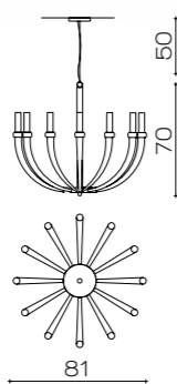
Art. 2071/CH12/BI ø 81 cm H 70 cm +50 cm steel cable 12 x G9 x Led 10W
