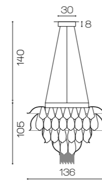
Art. 1984/G ø 136 cm H 105 cm +Ceiling plate ø 30 cm H 8 cm Steel cable 140 cm 12 x E27 x 60W +3 x GU10 Led 10W
