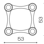
Art. 2195/BI L 53 x 53 cm H 3 cm H tot 25 cm G x 53 4 x 11W Led ø int. 75 mm
