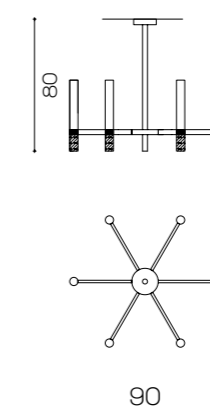
Art. 2173/CH6+6 ø 90 cm H 80 cm 12 x G9 x Led
