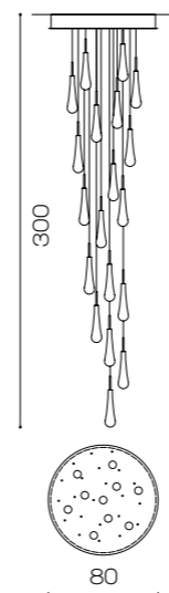
Art. 2183 ø 80 cm H 300 cm 22 x G9 x Led +10 x GU10 Led
