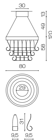
Art. 1937 Chandelier ø 80 cm H 58 cm +Ceiling plate H 13 cm ø 30 cm with 3 GU10 Led 10W H tot. 120 cm +Strip Led Colour light 2700 K° Lumen 8550
