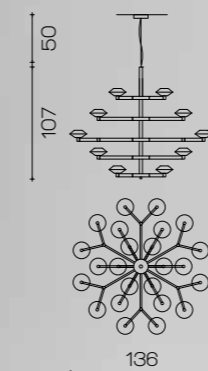
Art. 2129/CH36/SG ø 136 cm H 107 cm 36 x G9 x Led 10W
