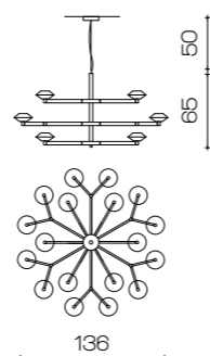
Art. 2129/CH24/SG ø 136 cm H 65 cm 24 x G9 x Led 10W
