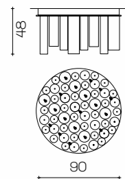
Art. 2078/Steel ø 90 cm H 48 cm 18 x G9 x 25W Steel
