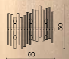
Art. 2054/A/NN L 60 cm H 55 cm Sp 12 cm 6 x G9 x Led max 10W
