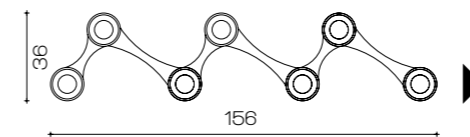
Art. 2200/BI/GOLD L 156 x 36 cm H 3 cm H tot 25 cm G x 53 7 x 11W Led ø int. 75 mm
