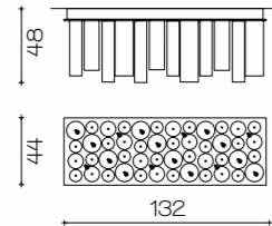
Art. 2077/Steel L 132 x 44 cm H 48 cm 18 x G9 x 25W Steel
