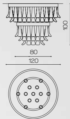
Art. 2015/NL ø 120 cm H 100 cm Lumen Colour light 2700 K° Lumen 7000 +12 x GU10 Led 5W (bulbs not included)
