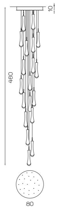
Art. 2181 ø 80 cm H 460 cm 22 x G9 x Led
