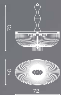
Art. 1820/CH ovale L 72 x 40 cm H 70 cm 4 x E27 x 60W
