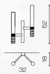
Art. 2173/A2+2 L 32 cm H 52 cm Sp 18 cm 4 x G9 x Led
