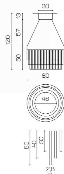
Art. 1971 ø 80 cm H 50 cm +Ceiling plate H 13 cm ø 30 cm with 3 GU10 Led 10W H tot. 120 cm Luce colore 2700°K Lumen 8550
