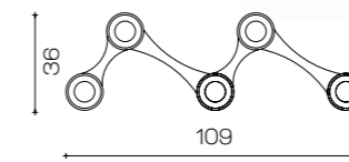
Art. 2199/BI L 109 x 36 cm H 3 cm H tot 25 cm G x 53 5 x 11W Led ø int. 75 mm
