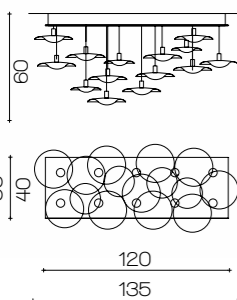
Art. 2059/Steel L 135 x 55 cm H 60 cm 10 x GU10 x 40W
