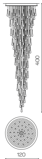
Art. 2023/CH40/LU ø 120 cm H 400 cm 40 x E14 x Led 5W
