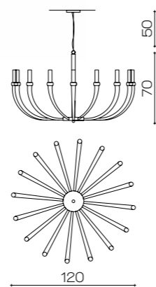
Art. 2071/CH16/BI ø 120 cm H 70 cm +50 cm steel cable 16 x G9 x Led 10W
