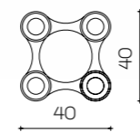
Art. 2196/BI L 40 x 40 cm H 3 cm H tot 25 cm G x 53 4 x 11W Led ø int. 75 mm
