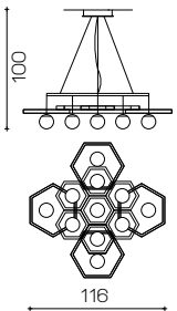
Art. 2123/CH11/LU ø 116 cm H tot. 100 cm 11 x G9 x Led 10W
