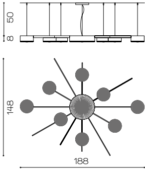
Art. 2166/CH30 L. 188 x 148 cm H 9 cm +50 steel cable 30 x G9 x Led
