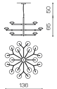
Art. 2129/CH24/SG ø 136 cm H 65 cm 24 x G9 x Led 10W
