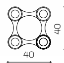
Art. 2196/B1 L 40 x 40 cm H 3 cm H tot 25 cm G x 53 4 x 11W Led ø int. 75 mm
