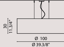
6 x E27 SUITABLE FOR LED LAMPS
