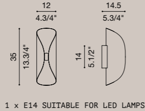
1 x E14 SUITABLE FOR LED LAMPS
