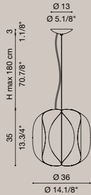
6 x E14 SUITABLE FOR LED LAMPS + 1 x GX53 / double light emission
