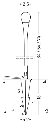
Mounting by spike
