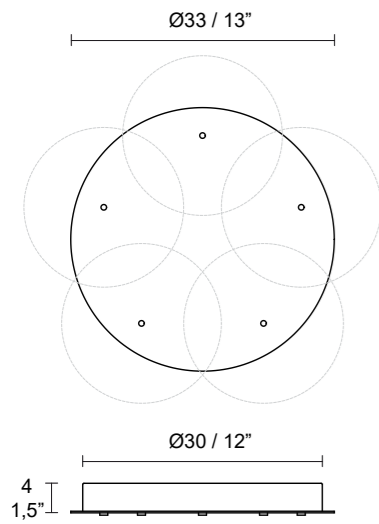
Rosoni multipli 5 Multiple canopies 5
