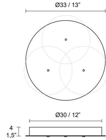
Rosoni multipli 3 Multiple canopies 3
