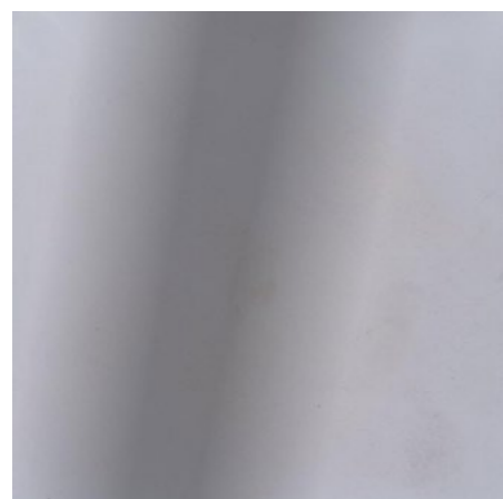
Cromo Chrome
