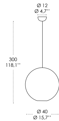
LD0516 LED DIMMER
